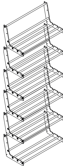
KIT 6 RIPIANI TUBI INCLINATI KIT 6 INCLINED TUBE SHELVES
